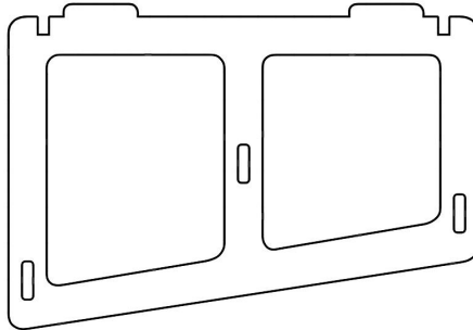
B) Platform Side Support (x2)
